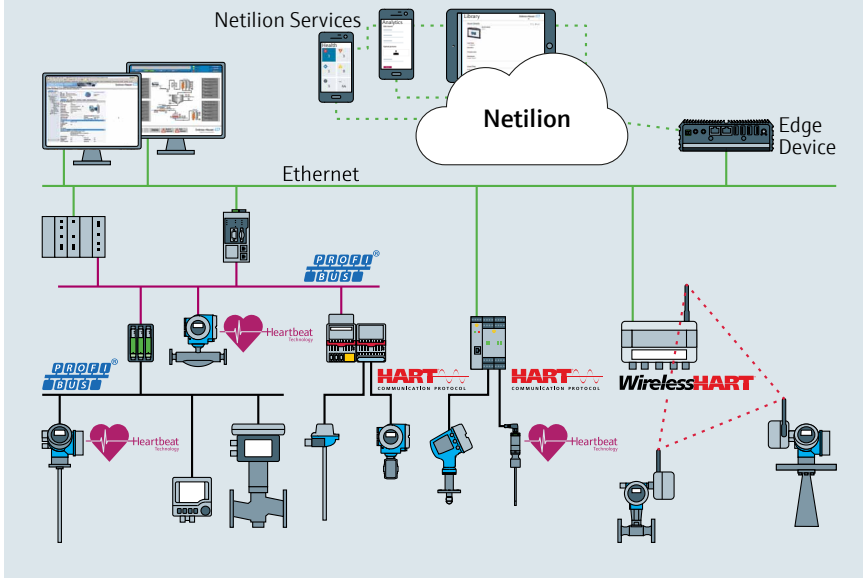
Our Edge Device and Gateways in action in industrial network topologies
